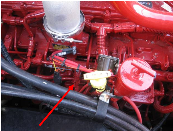
8.3 L & 9.0L Cummins Fuel Pressure Sensor in 88 series combine
